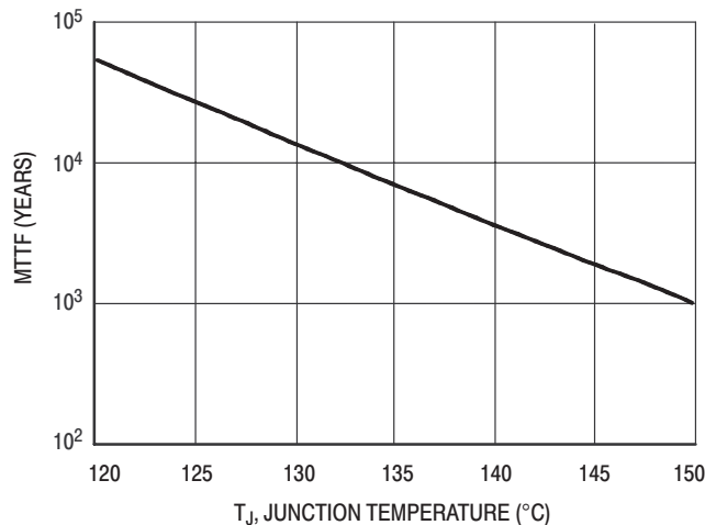
Figure 11. MTTF versus Junction Temperature NOTE: The MTTF is calculated with V_{CC} = 5.2 Vdc, I_{CC} = 110 mA
