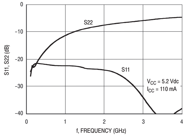
Figure 3. Unmatched Input/Output Return Loss versus Frequency
